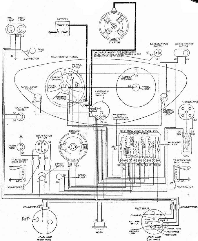
WIRING DIAGRAM FOR MORRIS EIGHT (SERIES "E") CARS (1945-46).
